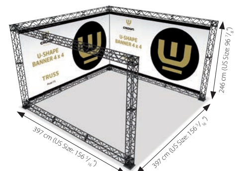
Truss U-Shape 4 x 4
